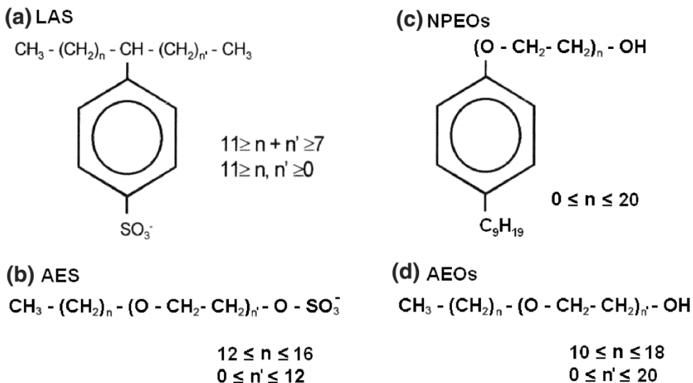
Figure 1. General chemical structures of (a) linear alkylbenzene sulfonate (LAS), (b) alkyl ethoxysulfate (AES), (c) nonylphenol polyethoxylates (NPEO) and (d) alcohol polyethoxylate (AEO) compounds.
