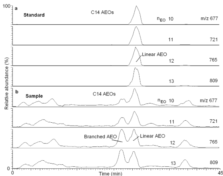
Figure 5. Extracted HPLC/MS ESI positive ion chromatograms showing the presence of linear and branched C_{14} AEOs ethoxymers with n_{EO} between 10 and 13 in (a) a standard solution and (b) a sediment sample. Chromatograms were obtained under the specific analytical conditions described in Section 2.4.
