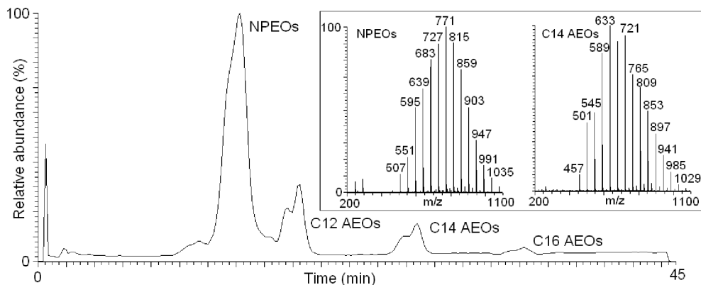
Figure 2. Full-scan HPLC/MS ESI positive ion chromatogram showing the separation between NPEOs and AEOs homologues in a standard solution. Also, mass spectra of NPEOs and C 14 AEOs are presented, showing the adduct ions [M+Na]^+ of the different ethoxymers. Chromatograms and mass spectra were obtained under specific analytical conditions described in Section 2.4.
