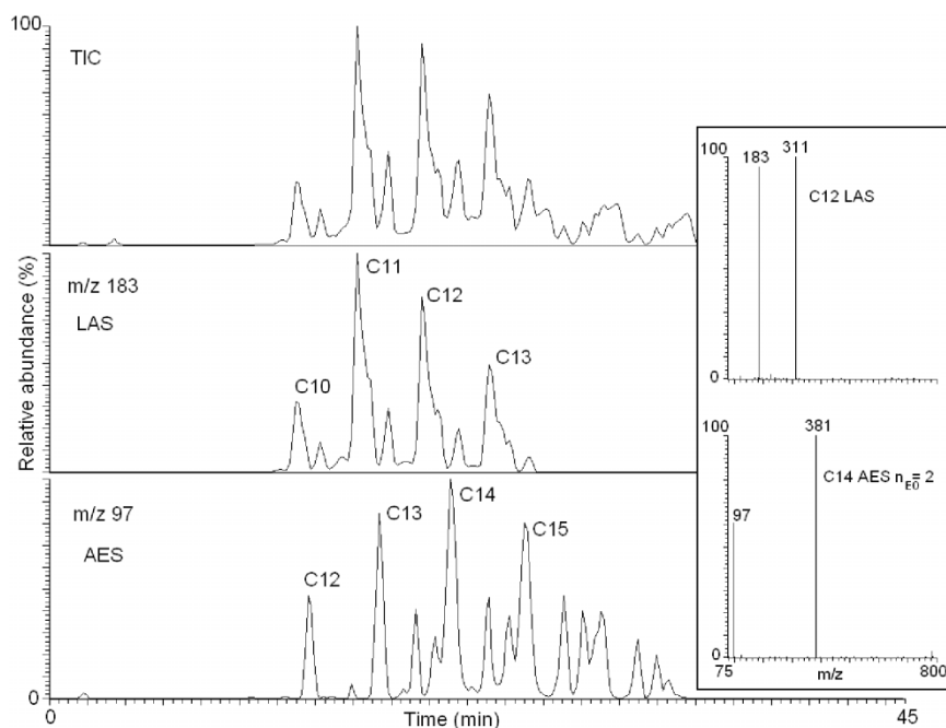
Figure 3. Full-scan HPLC/MS ESI negative ion chromatogram showing the presence of LAS and AES homologues in a standard solution. Also, two extracted ion chromatograms are presented, showing the separation between the homologues of these two surfactants by means of their specific fragment ions m/z 183, for LAS, and m/z 97, for AES. Mass spectra of C_{12} LAS and C_{14} AEOs with n_{EO}=2 are presented as examples. Chromatograms and mass spectra were obtained under the specific analytical conditions described in Section 2.4.
