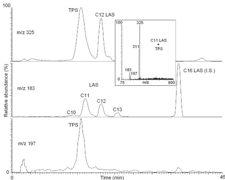
Figure 4. Extracted HPLC/MS ESI negative ion chromatograms showing the identification of tetrapropylenebenzenesulfonate (TPS) in a sediment sample among LAS homologues by means of its quasimolecular and specific fragments m/z 325 and 197, respectively. Also, a mass spectrum of TPS together with C_{11} LAS is presented. Chromatograms and mass spectra were obtained under specific analytical conditions described in Section 2.4.
